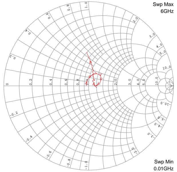
De-Embedded S22, V_{CC} = 4.84\text{V} , I_{CC} = 65\text{mA} , T = 25^\circ\text{C}
